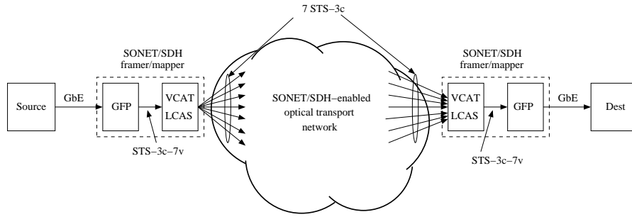
Fig. 1.6. Virtual concatenation for transport of Gigabit Ethernet (GbE)
