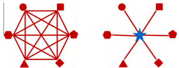
Fig. 1. Heterogeneity of parties leads to O(M^2) translators (left) or a layer of M translators (right).
